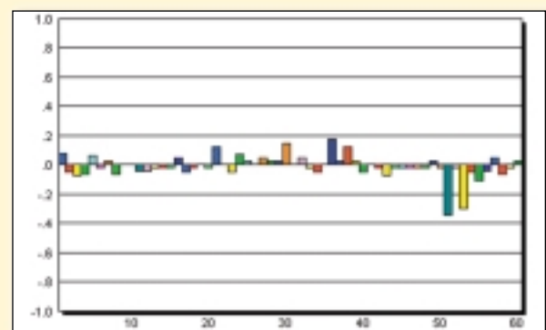
Typical Histogram
