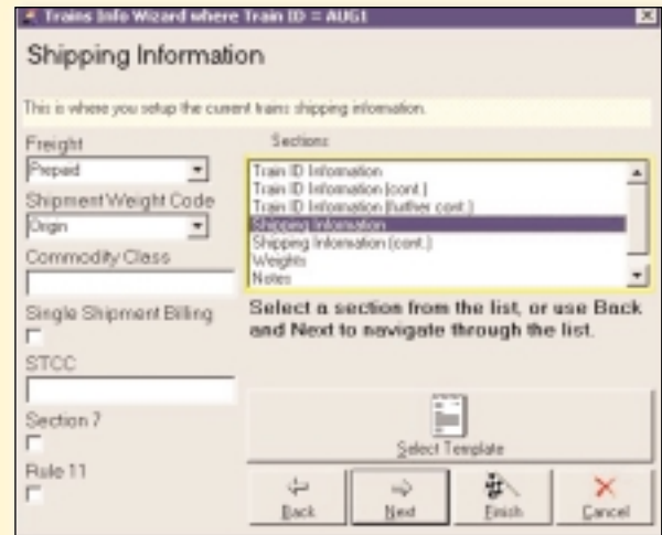
Setup Wizard
